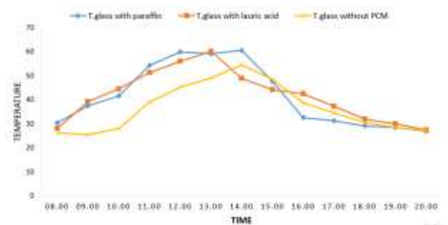
Fig. 8. Comparison of glass temperature versus time in the study of PCM paraffin, lauric acid, and without PCM
